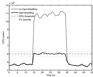
Fig. 4 CPU usage with and without load shedding
