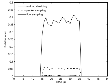
Fig. 5 Error in the query results with and without load shedding
