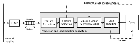
Fig. 2 Prediction and load shedding system
